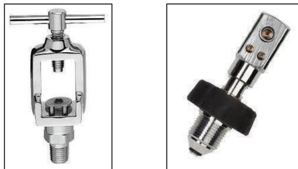
Pin-indexed medical post outlet (L), threaded outlet (R)
