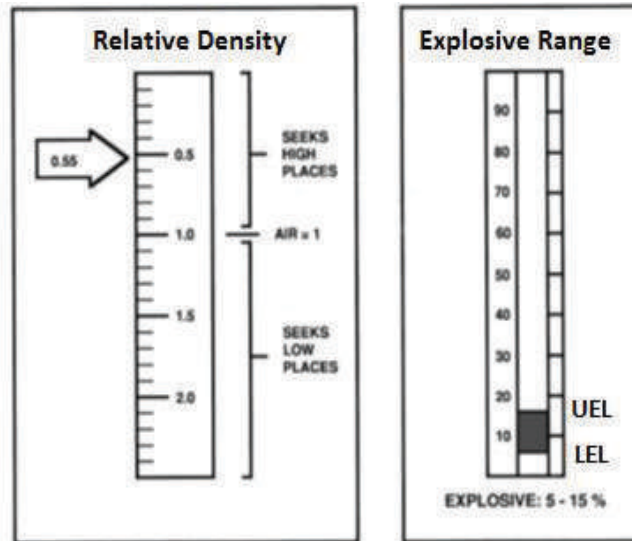
Fig 5.1 Relative density and Explosive range for Methane
